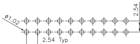
RECOMMENDED PCB LAYOUT (TOLERANCE:±0.10)
